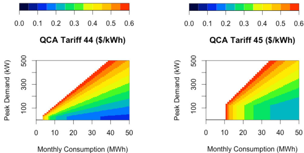
Figure 25. QCA Tariff 44 and 45 heat maps
