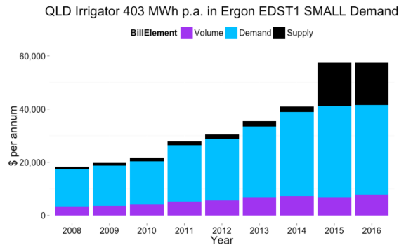
Figure 37. QLD Irrigator 403 MWh p.a. network average price (EDST1)
