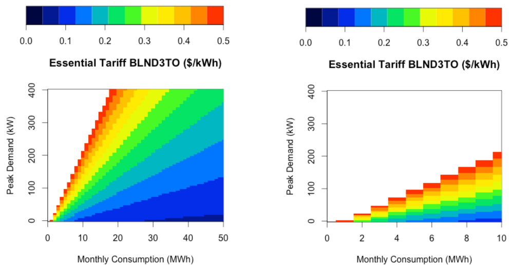
Figure 11. Heat maps for BLND3TO (a) 0 - 50 MWh per month (b) 0 - 10 MWh per month
