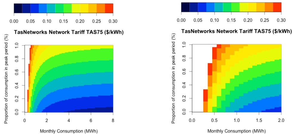
Figure 16. TasNetworks TAS75 Irrigation Tariff - for 20% consumption in the shoulder period. (a) 0 – 8 MWh p.a. and (b) 0 – 2 MWh p.a.
