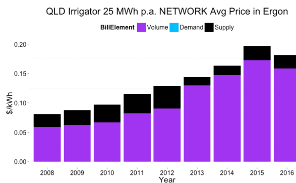
Figure 35. QLD Irrigator 25 MWh p.a. network bill breakdown
