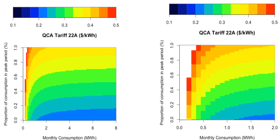
Figure 21. QCA Tariff 22A (a) 0 - 8 MWh per month (b) 0 - 2 MWh per month
