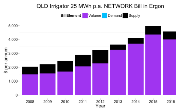
Figure 34. QLD Irrigator 25 MWh p.a. network average price
