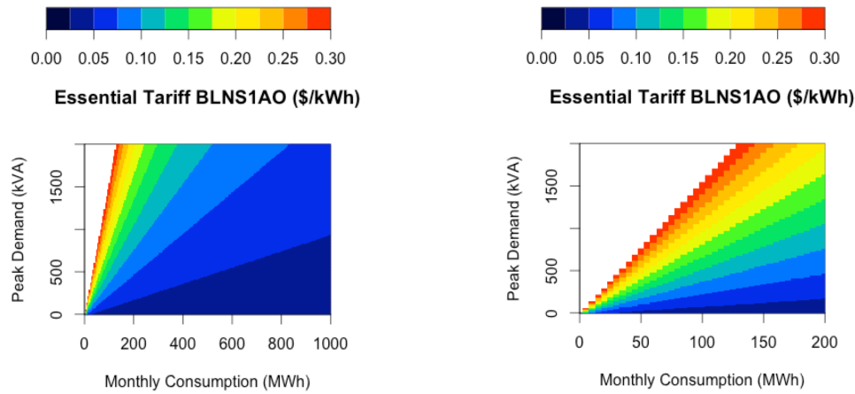
Figure 12. Heat maps BLNS1AO (a) 0 - 1000 MWh per month and (b) 0 - 200 MWh per month
