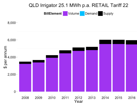
Figure 52. QLD Irrigator 25 MWh p.a. retail average price (Tariff 22)
